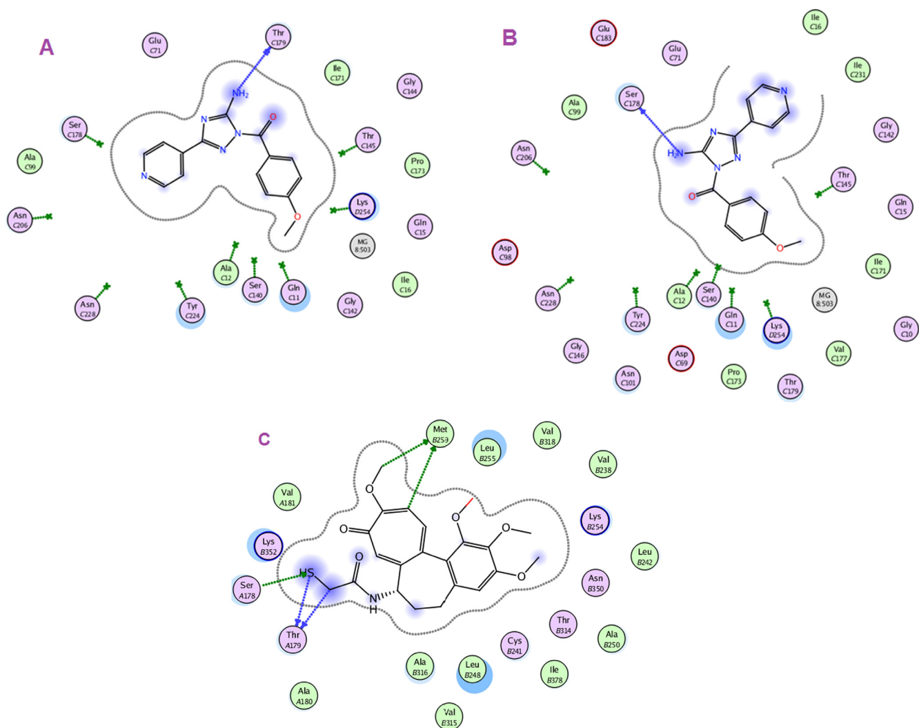
Fig. 4. (A and B) Docking and binding pattern of compound 8d into ATP-active site of tubulin (PDB code: isa0). (C) Docking and binding pattern of colchicine into ATP-active site of tubulin.
